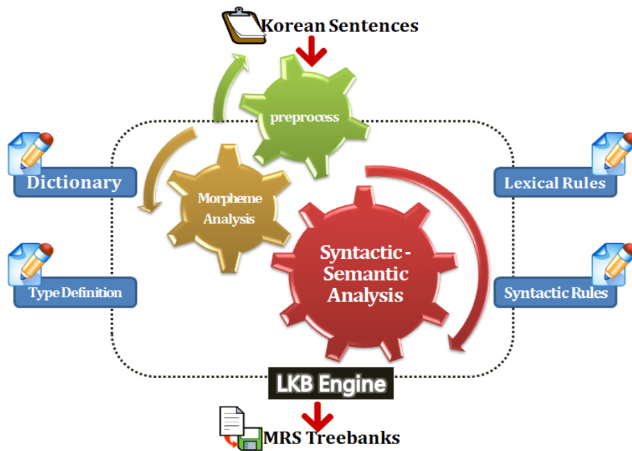
Figure 2: Main Components of the KRG
